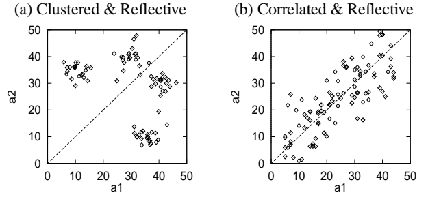
Figure 3: Counter-examples showing clustered and correlated datasets that are reflective.
