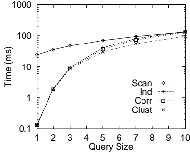
(a) Varying query size (#documents = 10K, #attributes = 20)
